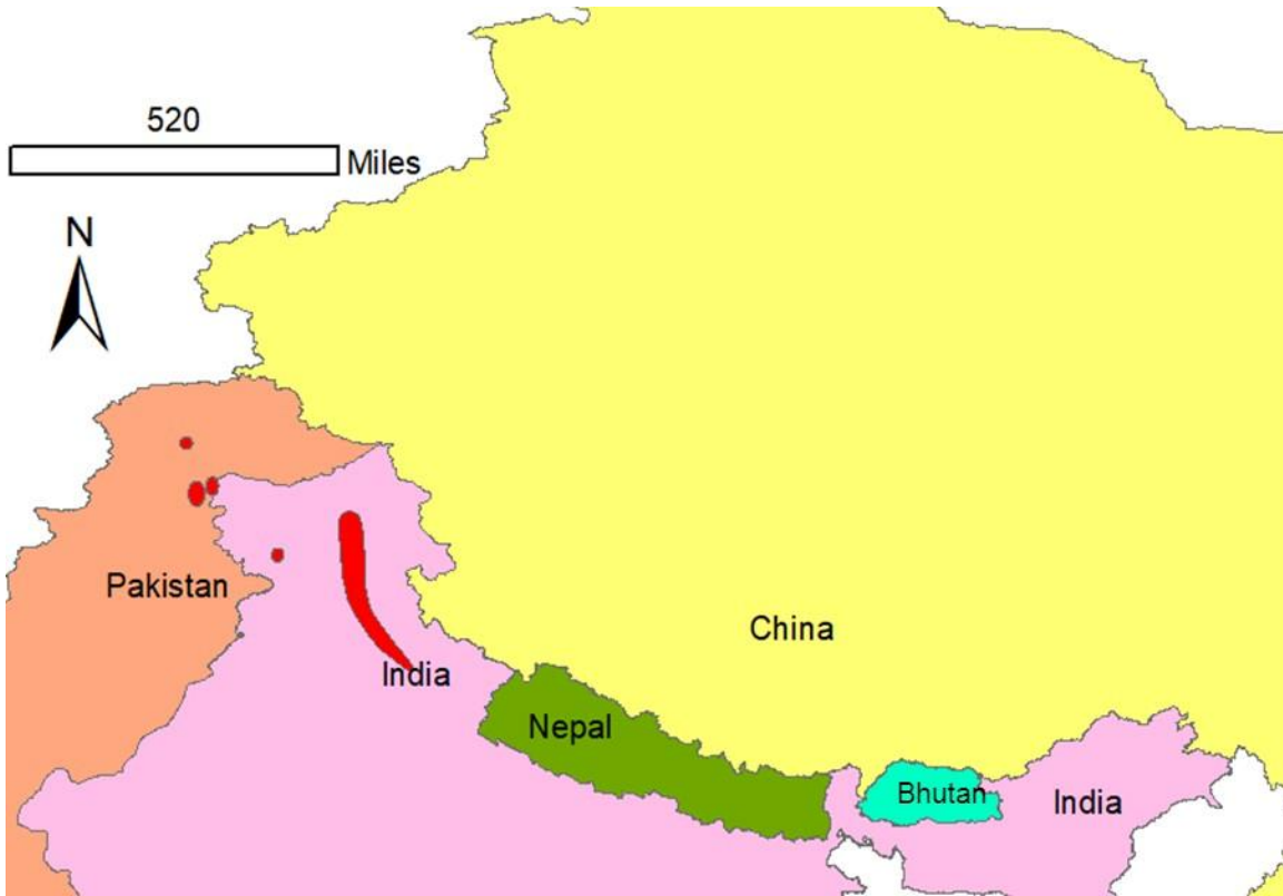
Figure S2. Map showing the BirdLife International range map of Tragopan melanocephalus (Western Tragopan).
